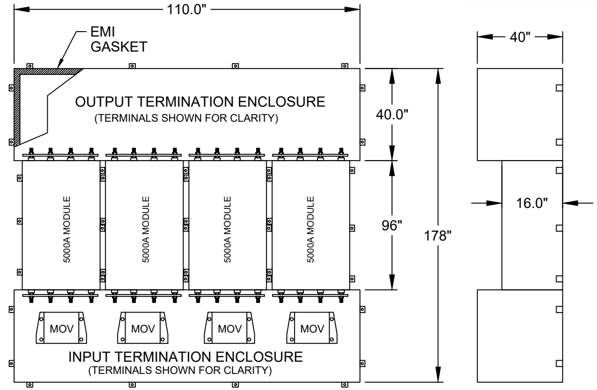
PER LINE END VIEW
